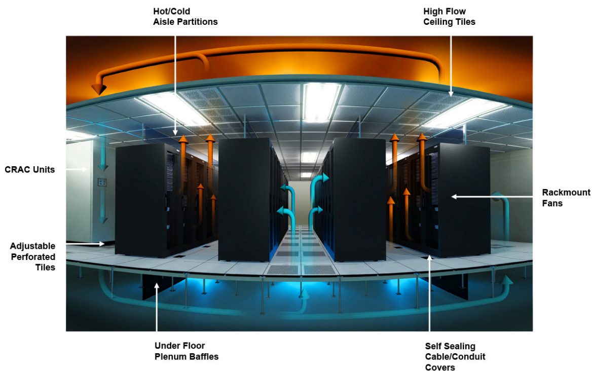
Figure 2. Simple and inexpensive airflow management practices can produce significant savings.
